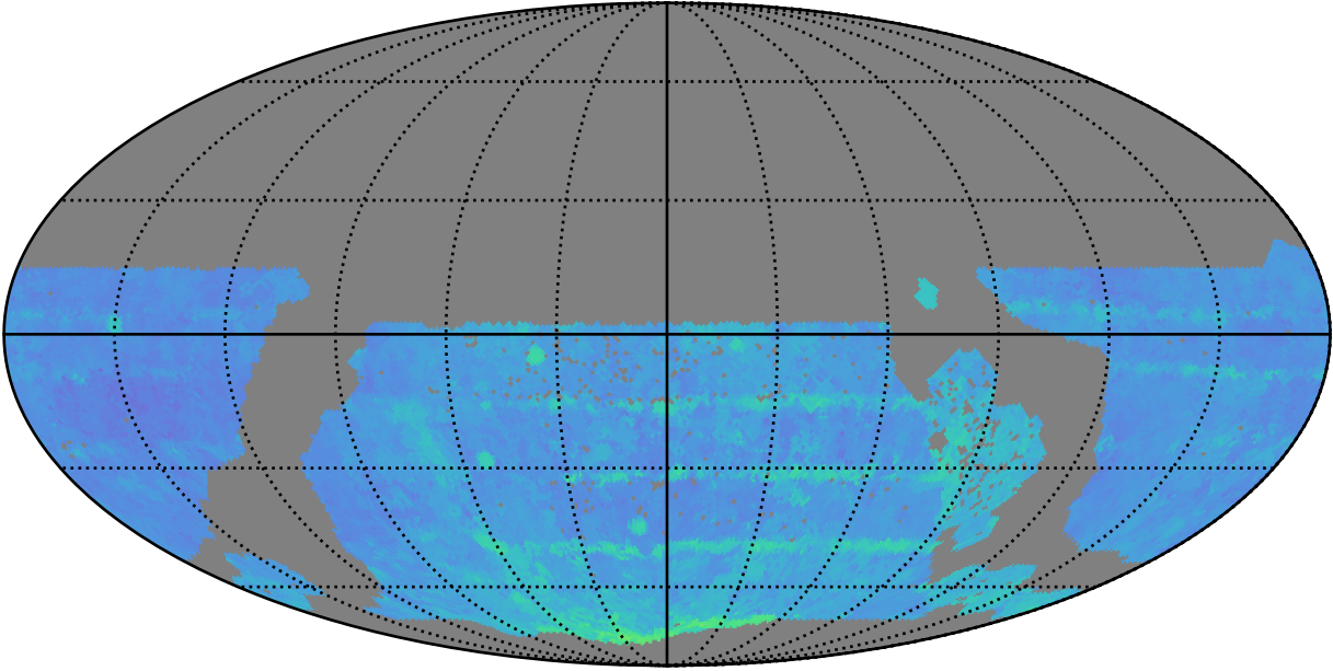
ddf_acor_sf15_lsf20_lsr10_v3.4_10yrs WFD i band: 80thPercentile Season Length
