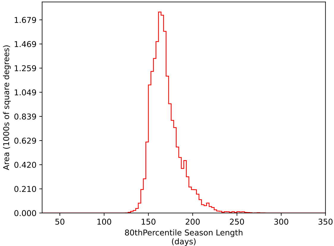
ddf_acor_sf15_lsf20_lsr10_v3.4_10yrs WFD i band: 80thPercentile Season Length
