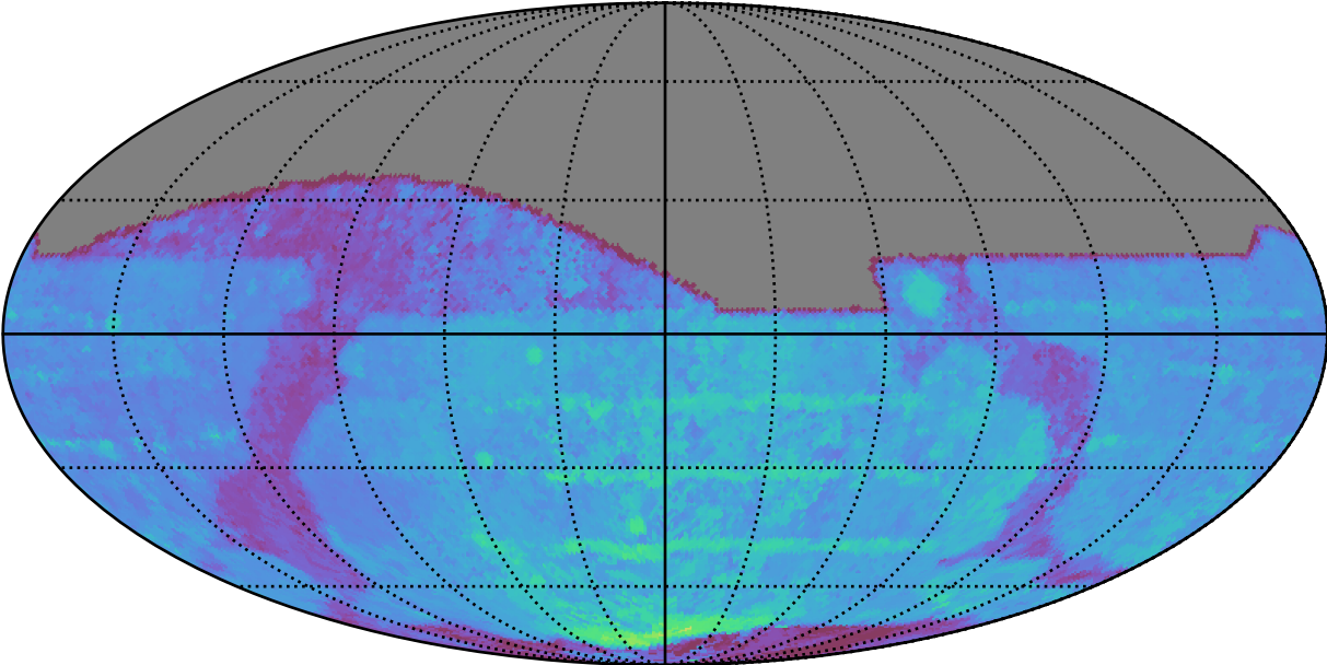
ddf_acor_sf15_lsf20_lsr10_v3.4_10yrs All sky z band: 80thPercentile Season Length
