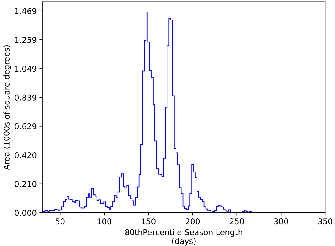
ddf_acor_sf15_lsf20_lsr10_v3.4_10yrs All sky y band: 80thPercentile Season Length
