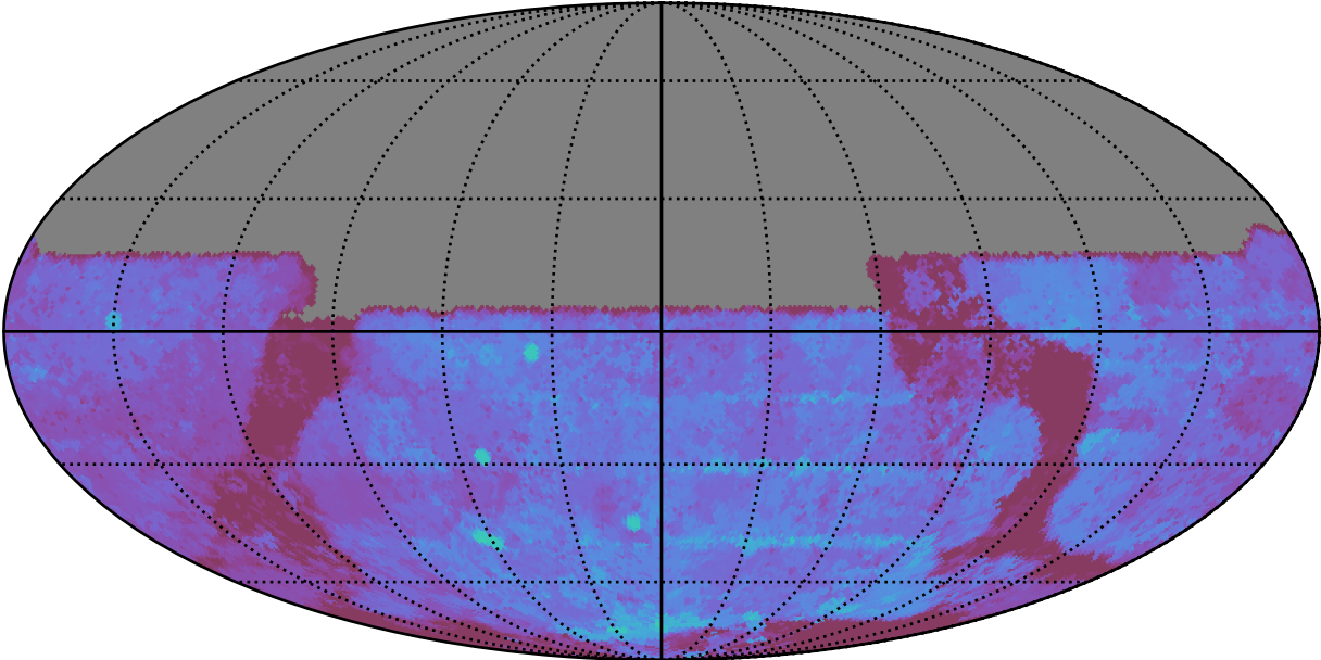
ddf_acor_sf15_lsf20_lsr10_v3.4_10yrs All sky u band: 80thPercentile Season Length
