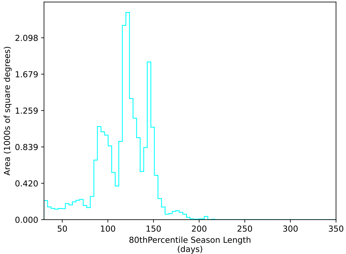
ddf_acor_sf15_lsf20_lsr10_v3.4_10yrs All sky u band: 80thPercentile Season Length
