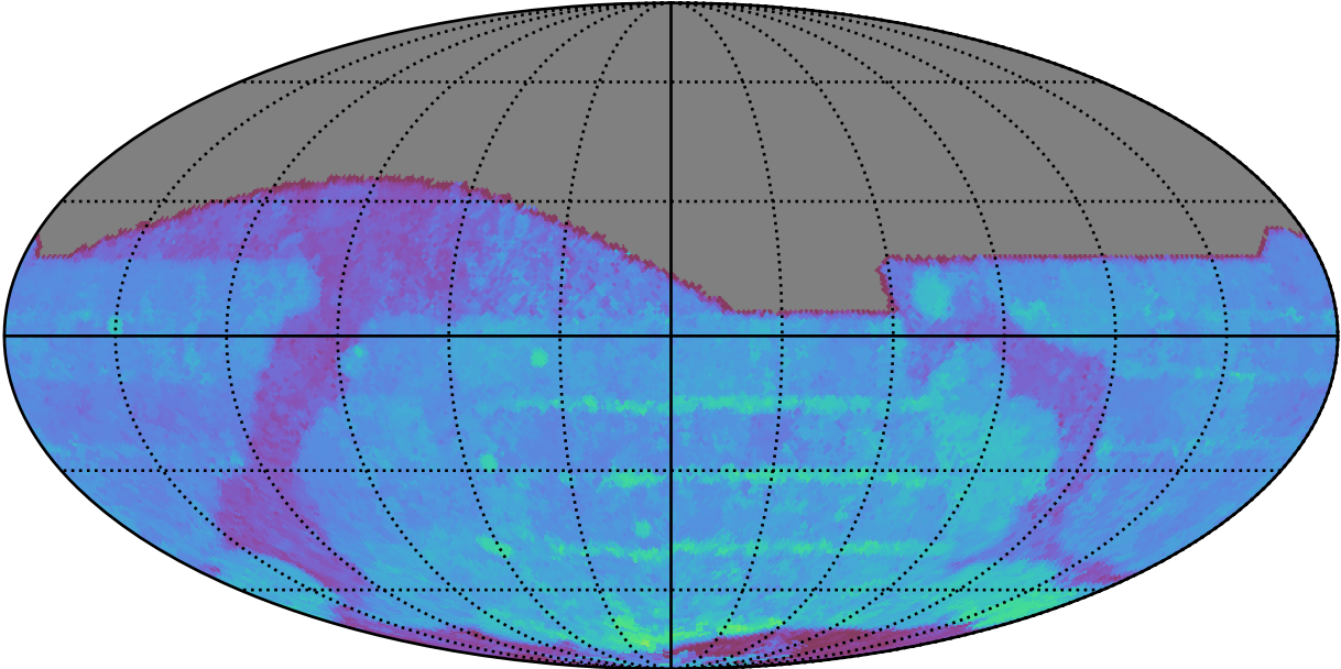
ddf_acor_sf15_lsf20_lsr10_v3.4_10yrs All sky r band: 80thPercentile Season Length
