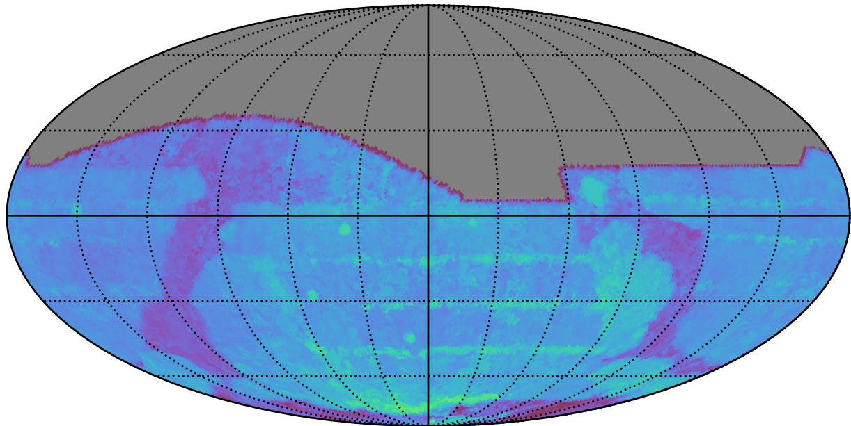
ddf_acor_sf15_lsf20_lsr10_v3.4_10yrs All sky i band: 80thPercentile Season Length
