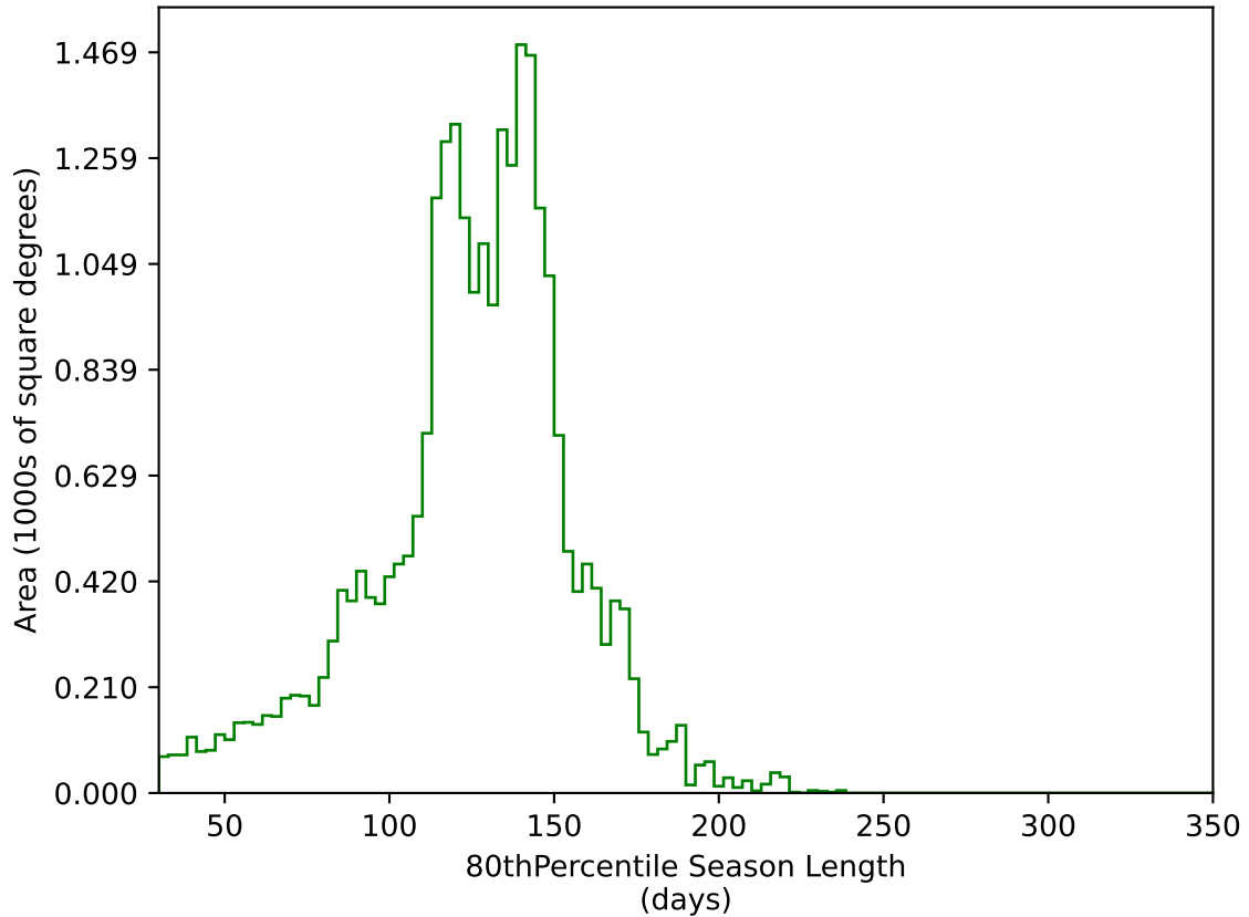
ddf_acor_sf15_lsf20_lsr10_v3.4_10yrs All sky g band: 80thPercentile Season Length
