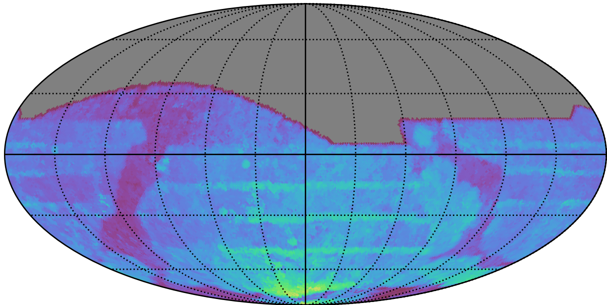
ddf_acor_sf15_lsf20_lsr10_v3.4_10yrs All sky all bands: 80thPercentile Season Length
