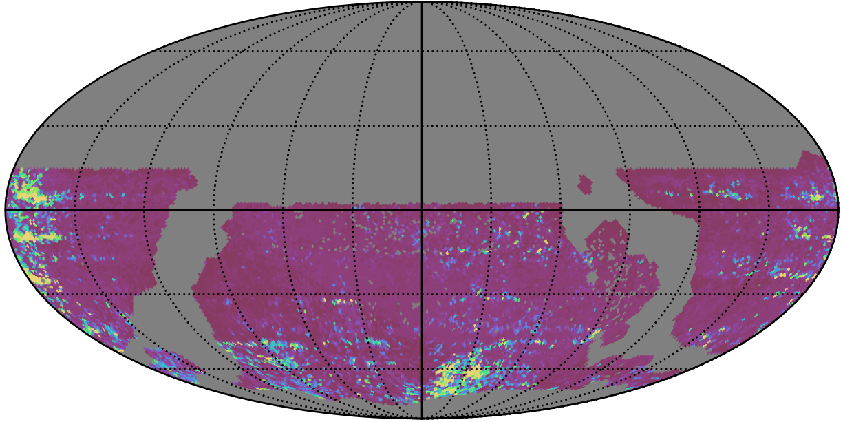
ddf_acor_sf15_lsf20_lsr10_v3.4_10yrs WFD z band: 75th Percentile Intranight Timespan
