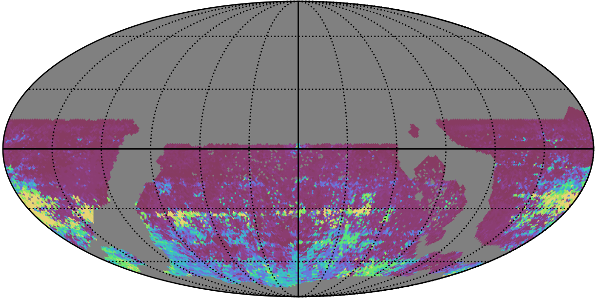
ddf_acor_sf15_lsf20_lsr10_v3.4_10yrs WFD r band: 75th Percentile Intranight Timespan
