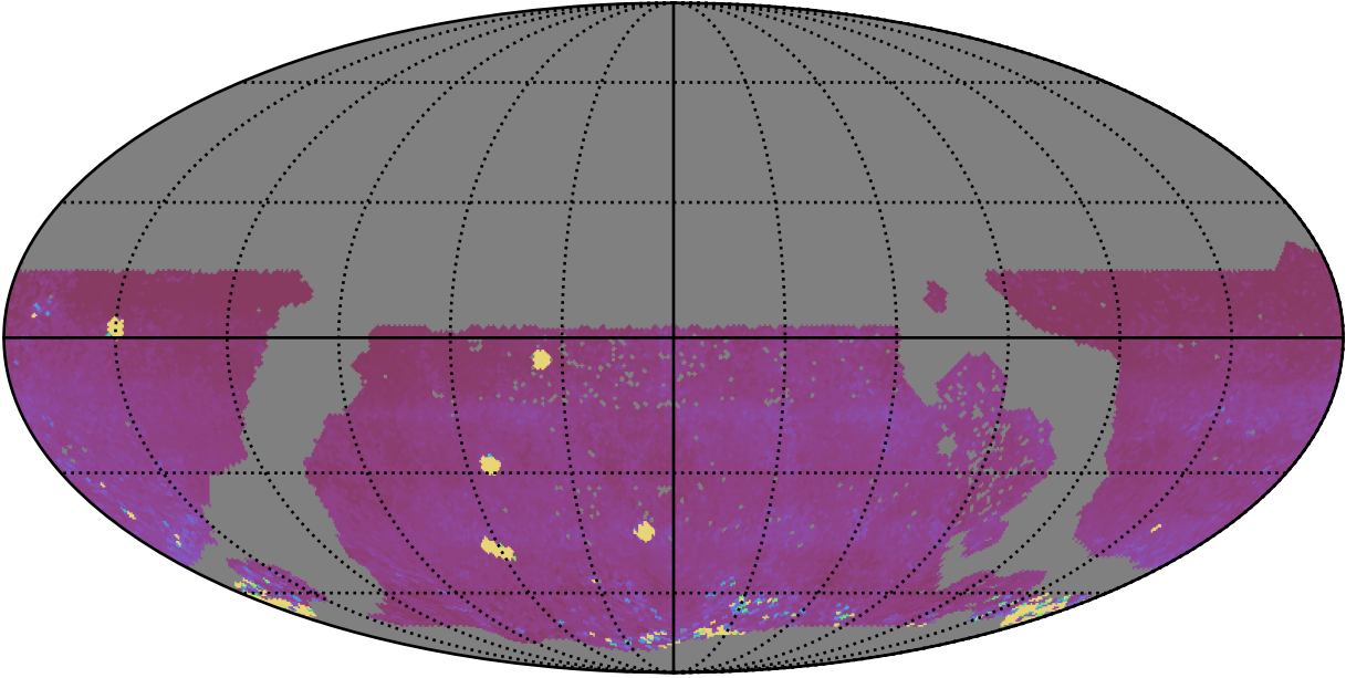
ddf_acor_sf15_lsf20_lsr10_v3.4_10yrs WFD iz bands: 75th Percentile Intranight Timespan
