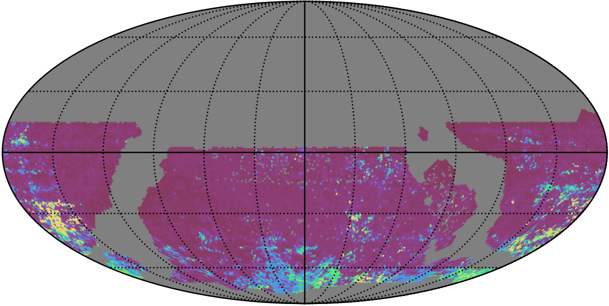
ddf_acor_sf15_lsf20_lsr10_v3.4_10yrs WFD i band: 75th Percentile Intranight Timespan
