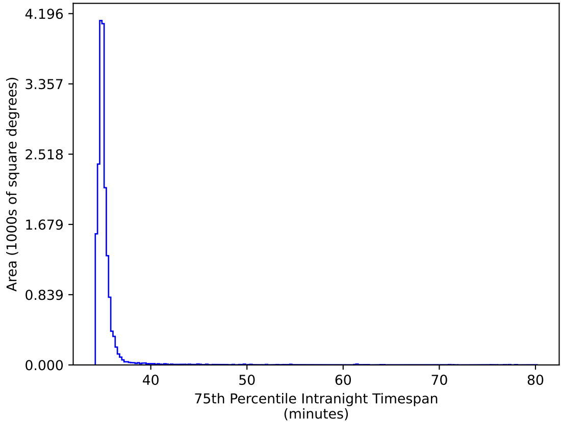
ddf_acor_sf15_lsf20_lsr10_v3.4_10yrs WFD gr bands: 75th Percentile Intranight Timespan
