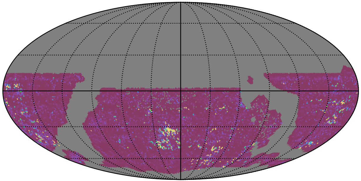
ddf_acor_sf15_lsf20_lsr10_v3.4_10yrs WFD g band: 75th Percentile Intranight Timespan
