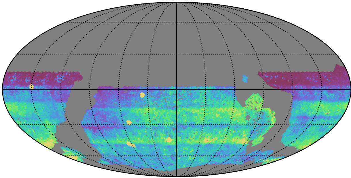
ddf_acor_sf15_lsf20_lsr10_v3.4_10yrs WFD all bands: 75th Percentile Intranight Timespan
