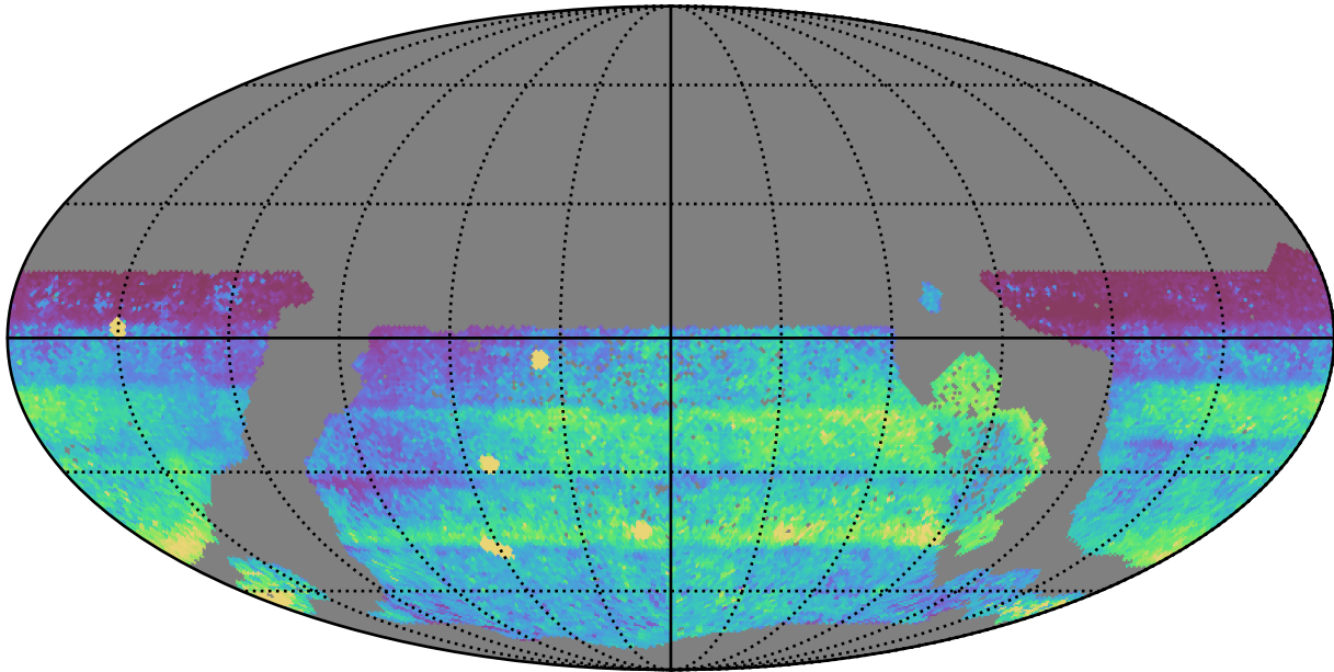
ddf_acor_sf15_lsf20_lsr10_v3.4_10yrs WFD: 75th Percentile Intranight Timespan
