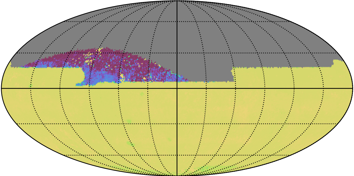
ddf_acor_sf15_lsf20_lsr10_v3.4_10yrs All sky zy bands: 75th Percentile Intranight Timespan
