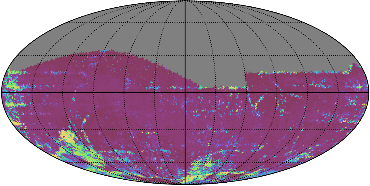
ddf_acor_sf15_lsf20_lsr10_v3.4_10yrs All sky z band: 75th Percentile Intranight Timespan
