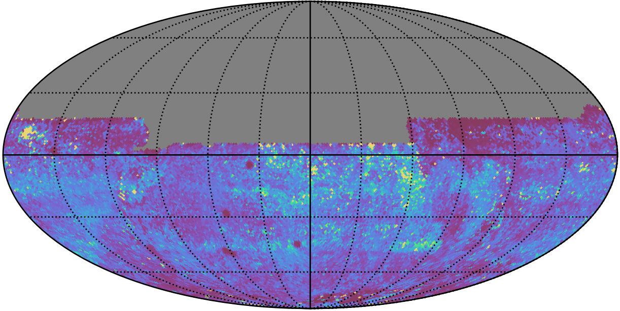
ddf_acor_sf15_lsf20_lsr10_v3.4_10yrs All sky y band: 75th Percentile Intranight Timespan
