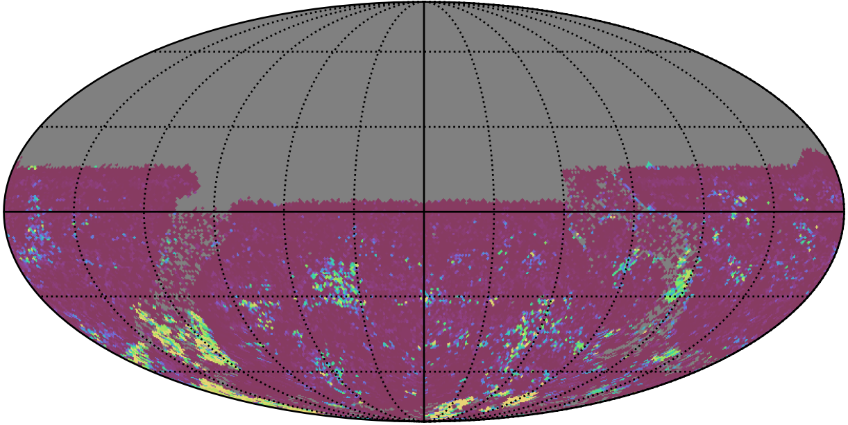
ddf_acor_sf15_lsf20_lsr10_v3.4_10yrs All sky u band: 75th Percentile Intranight Timespan
