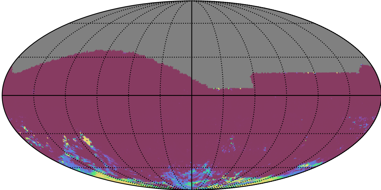
ddf_acor_sf15_lsf20_lsr10_v3.4_10yrs All sky ri bands: 75th Percentile Intranight Timespan
