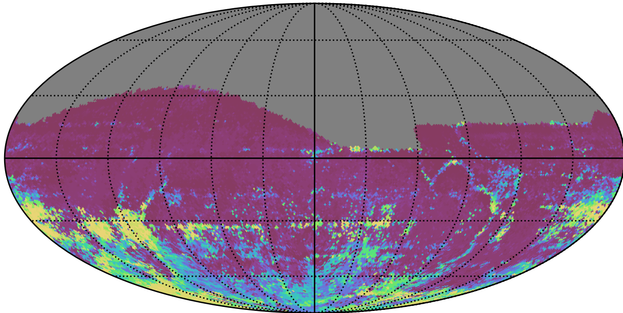
ddf_acor_sf15_lsf20_lsr10_v3.4_10yrs All sky r band: 75th Percentile Intranight Timespan
