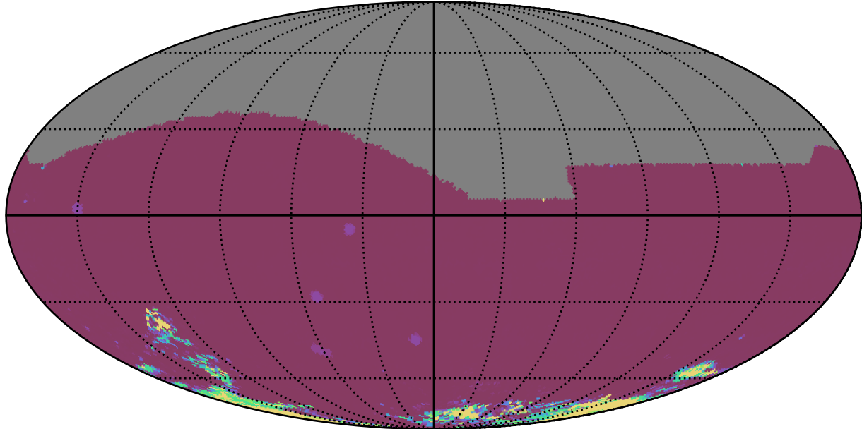
ddf_acor_sf15_lsf20_lsr10_v3.4_10yrs All sky iz bands: 75th Percentile Intranight Timespan
