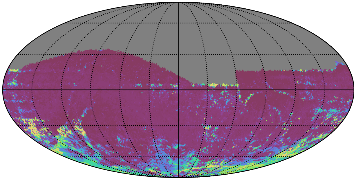
ddf_acor_sf15_lsf20_lsr10_v3.4_10yrs All sky i band: 75th Percentile Intranight Timespan
