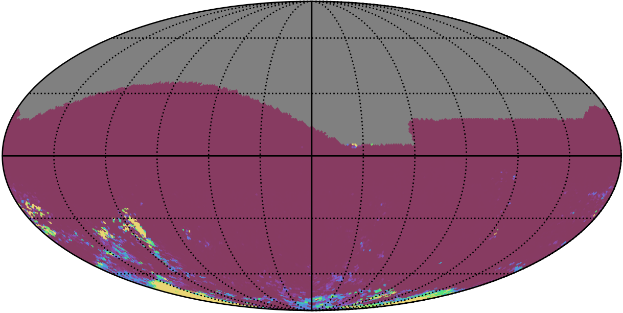
ddf_acor_sf15_lsf20_lsr10_v3.4_10yrs All sky gr bands: 75th Percentile Intranight Timespan
