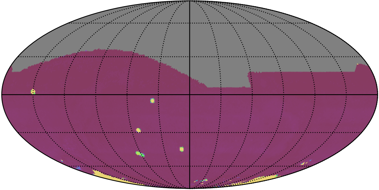
ddf_acor_sf15_lsf20_lsr10_v3.4_10yrs All sky all bands: 75th Percentile Intranight Timespan
