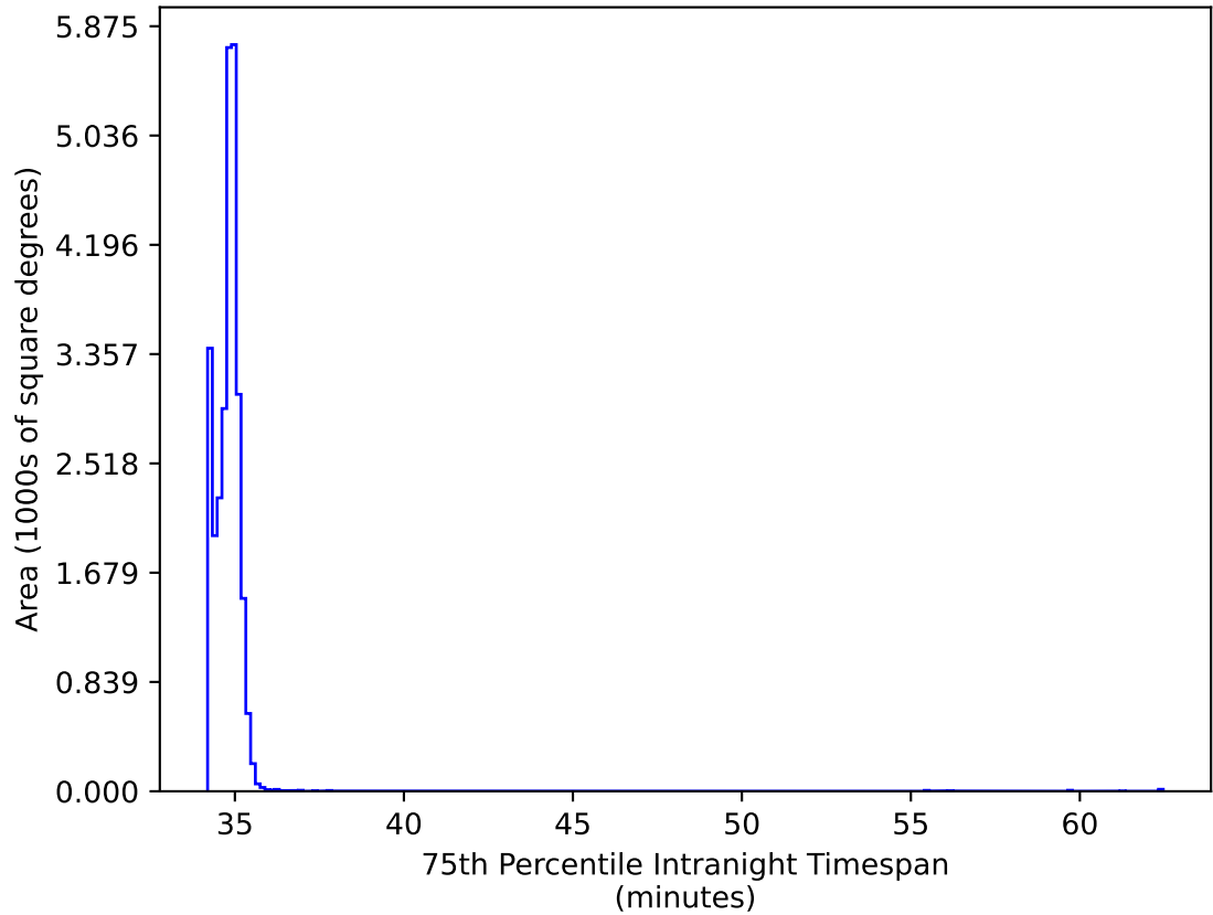
ddf_acor_sf15_lsf20_lsr10_v3.4_10yrs All sky: 75th Percentile Intranight Timespan
