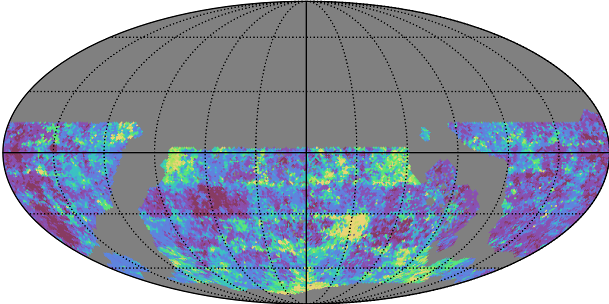
ddf_acor_sf15_lsf20_lsr10_v3.4_10yrs WFD g band: 20thPercentile Inter-Night Gap
