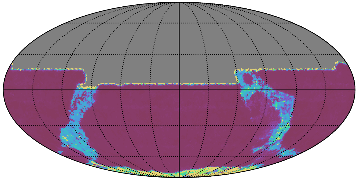
ddf_acor_sf15_lsf20_lsr10_v3.4_10yrs All sky y band: 20thPercentile Inter-Night Gap
