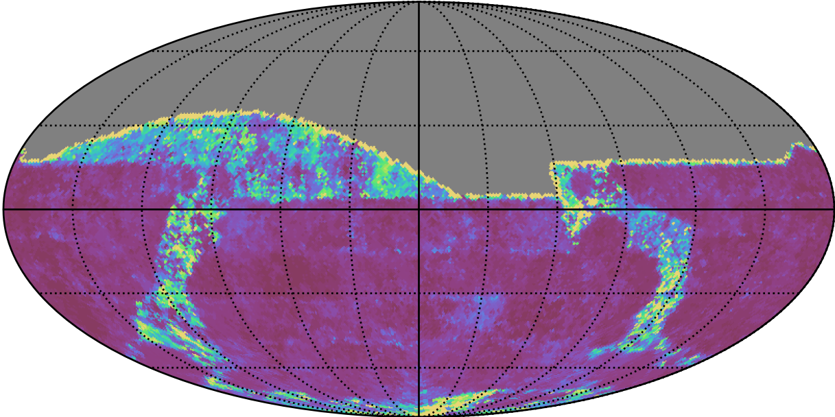
ddf_acor_sf15_lsf20_lsr10_v3.4_10yrs All sky g band: 20thPercentile Inter-Night Gap
