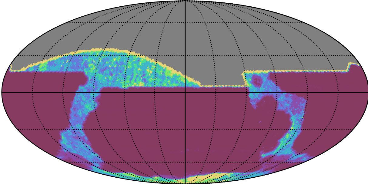
ddf_acor_sf15_lsf20_lsr10_v3.4_10yrs All sky all bands: 20thPercentile Inter-Night Gap
