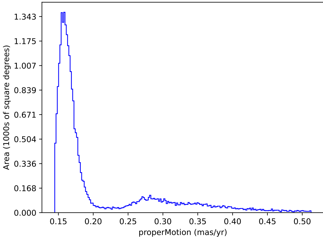
ddf_acor_sf15_lsf20_lsr10_v3.4_10yrs : properMotion
