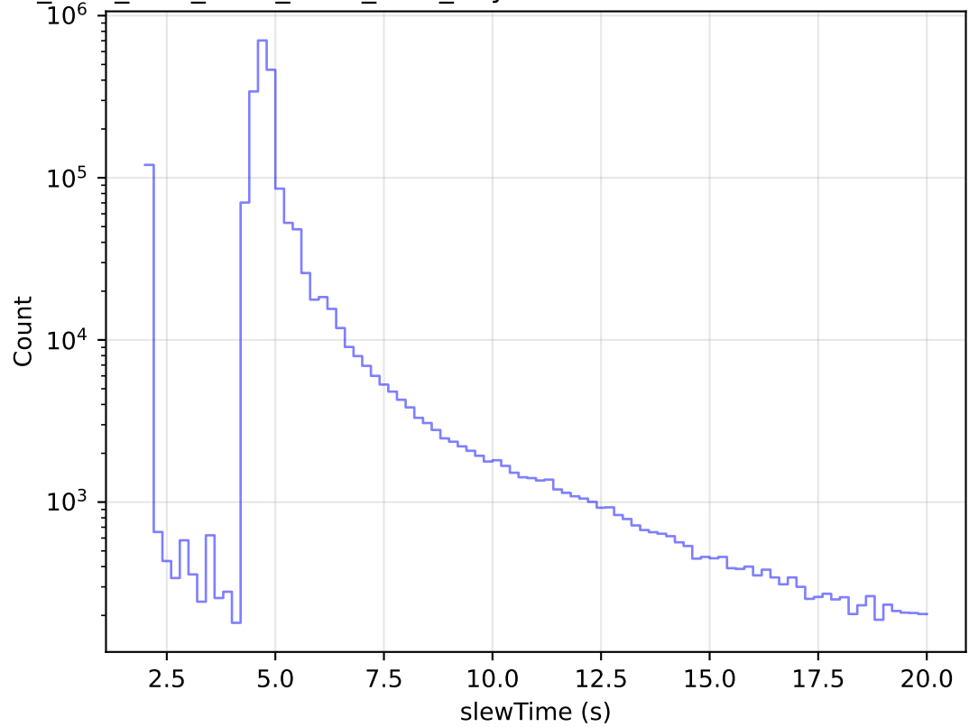
ddf_acor_sf15_Isf20_Isr10_v3.4_10yrs All visits: Zoom Slew Time Histogram
