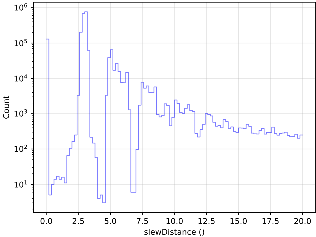
ddf_acor_sf15_lsf20_lsr10_v3.4_10yrs All visits: Zoom Slew Distance Histogram
