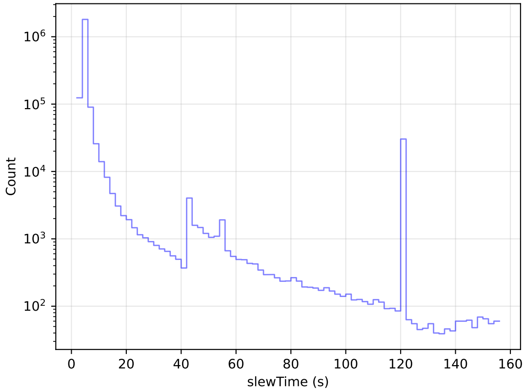
ddf_acor_sf15_lsf20_lsr10_v3.4_10yrs All visits: Slew Time Histogram
