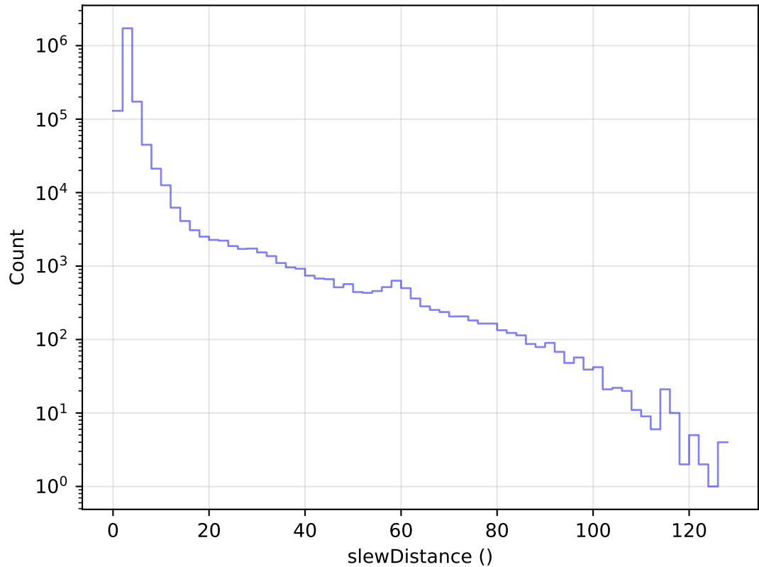
ddf_acor_sf15_lsf20_lsr10_v3.4_10yrs All visits: Slew Distance Histogram
