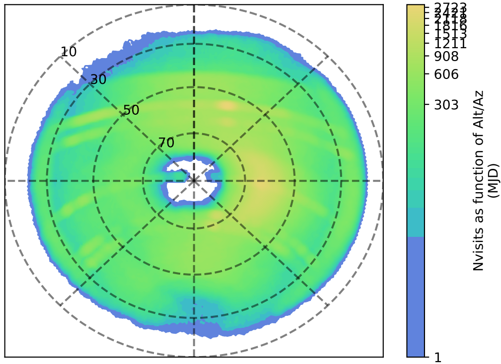
ddf_acor_sf15_lsf20_lsr10_v3.4_10yrs z: Nvisits as function of Alt/Az
