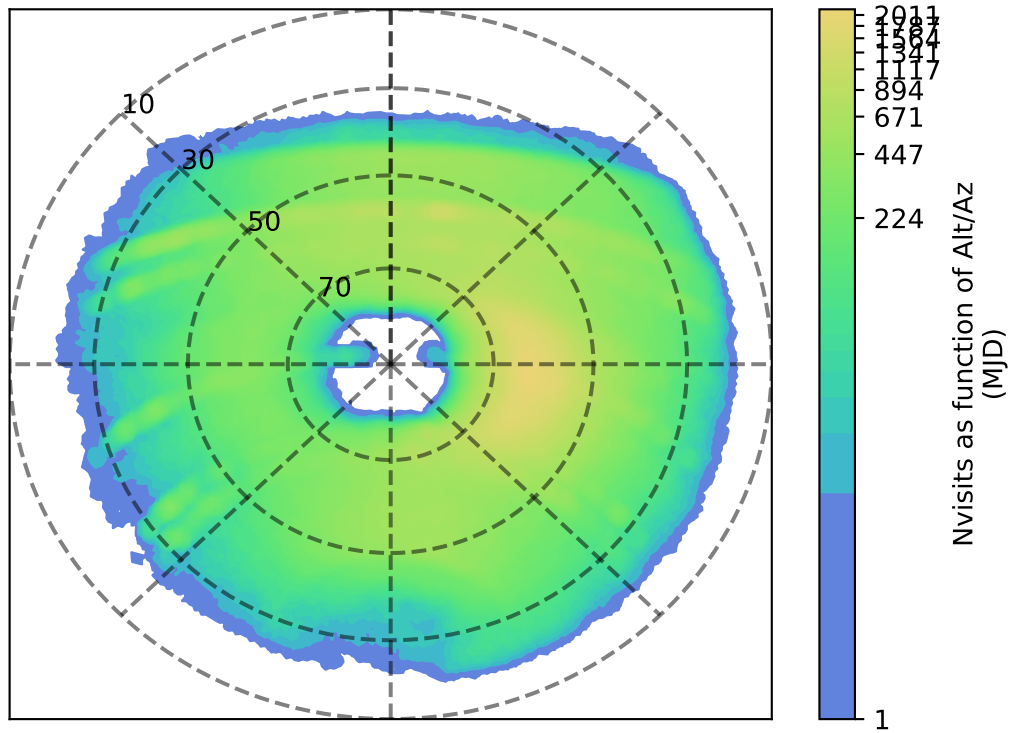
ddf_acor_sf15_lsf20_lsr10_v3.4_10yrs y: Nvisits as function of Alt/Az
