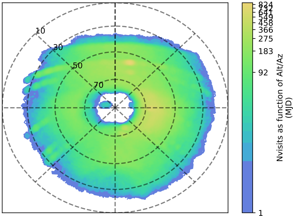
ddf_acor_sf15_lsf20_lsr10_v3.4_10yrs u: Nvisits as function of Alt/Az
