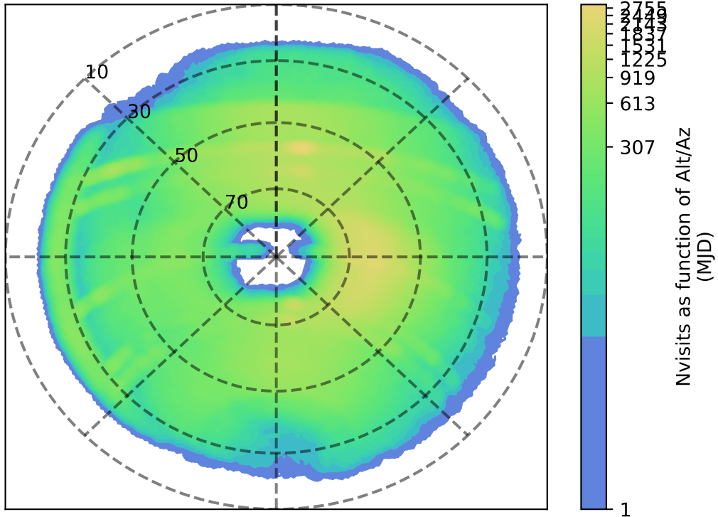
ddf_acor_sf15_ls20_lsr10_v3.4_10yrs r: Nvisits as function of Alt/Az
