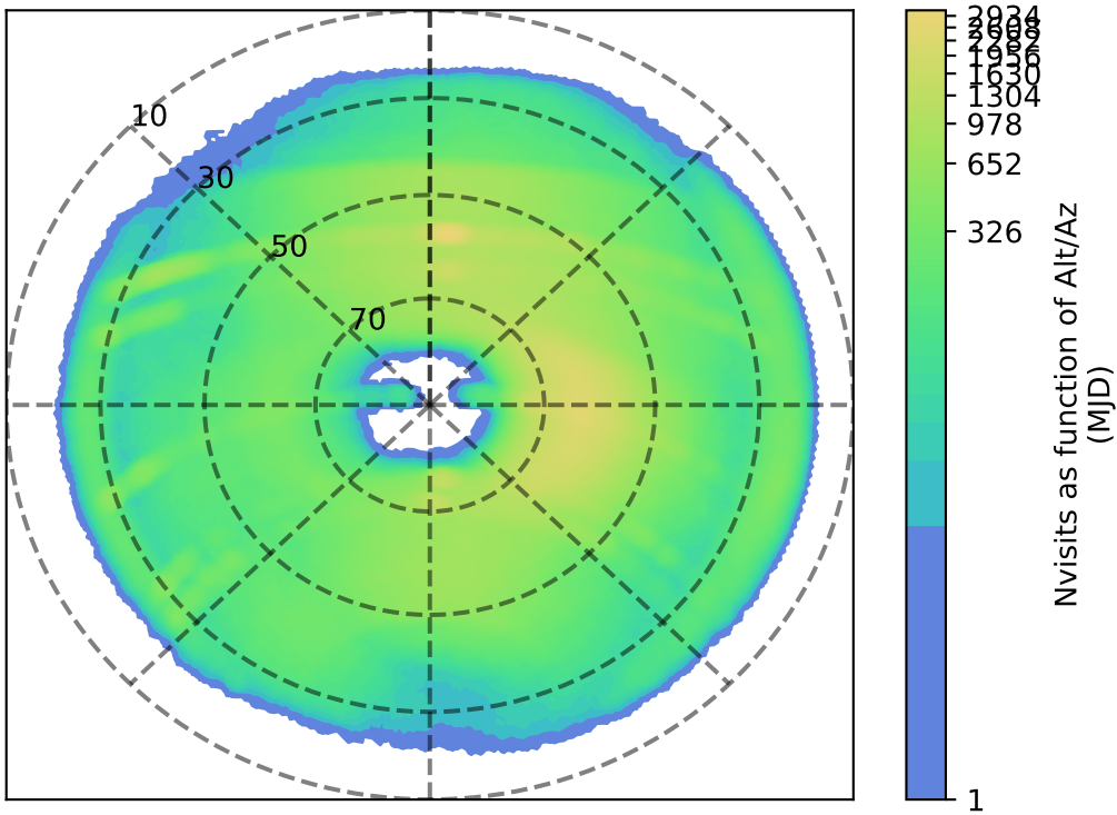
ddf_acor_sf15_ls20_lsr10_v3.4_10yrs i: Nvisits as function of Alt/Az
