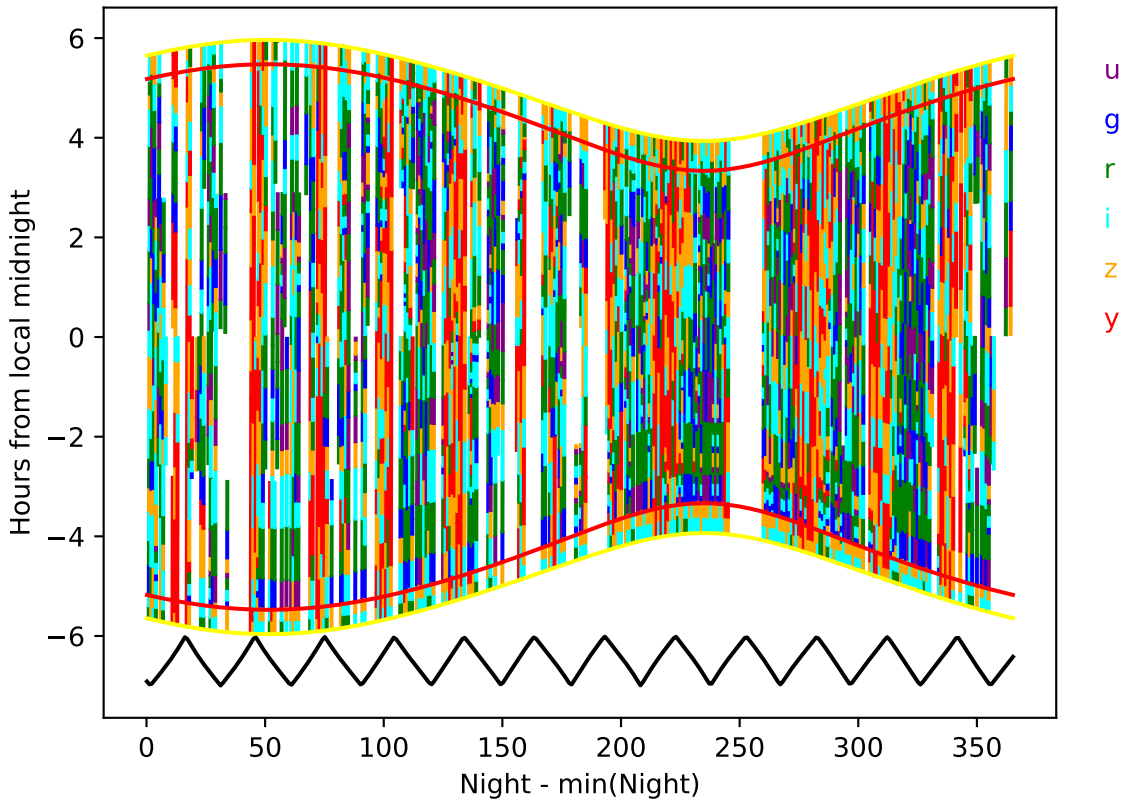
ddf_acor_sf15_lsf20_lsr10_v3.4_10yrs year 5-6: Hourglass
