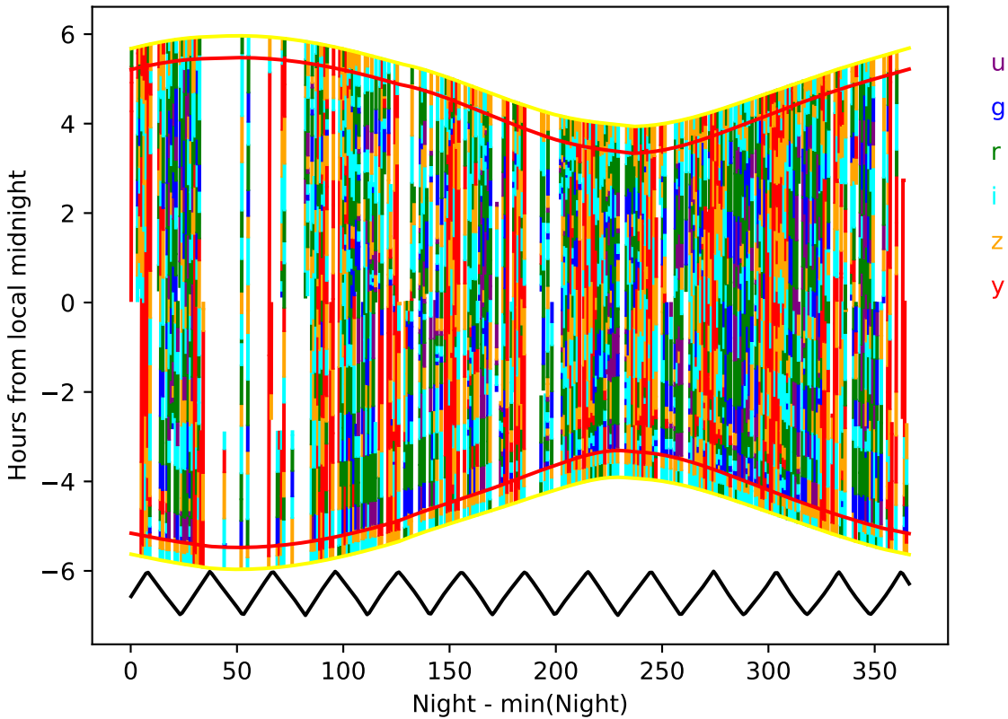
ddf_acor_sf15_lsf20_lsr10_v3.4_10yrs year 3-4: Hourglass
