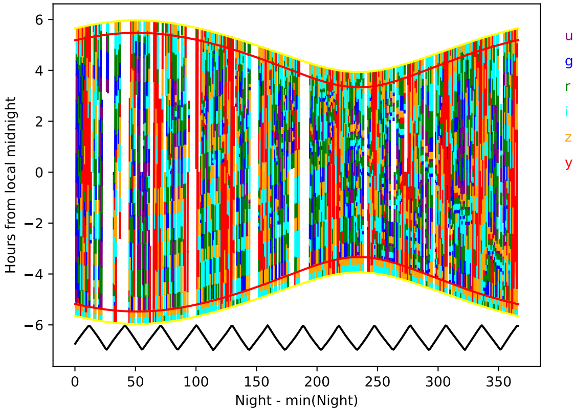
ddf_acor_sf15_lsf20_lsr10_v3.4_10yrs year 0-1: Hourglass
