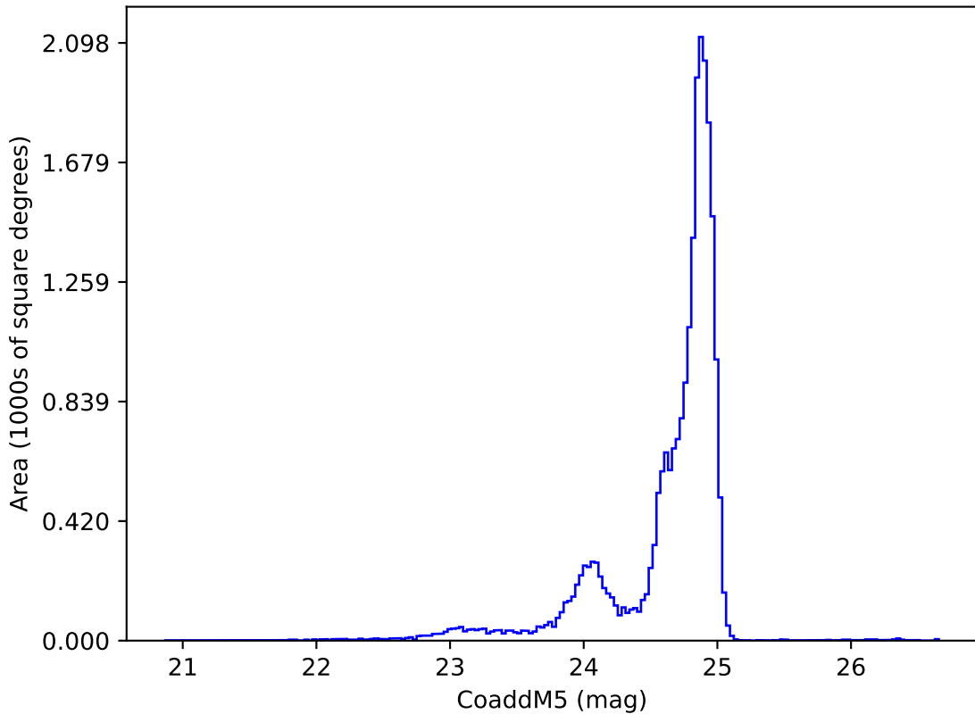
ddf_acor_sf15_lsf20_lsr10_v3.4_10yrs y: CoaddM5
