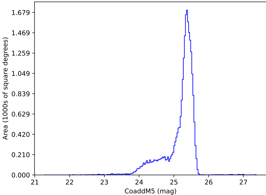
ddf_acor_sf15_lsf20_lsr10_v3.4_10yrs u: CoaddM5
