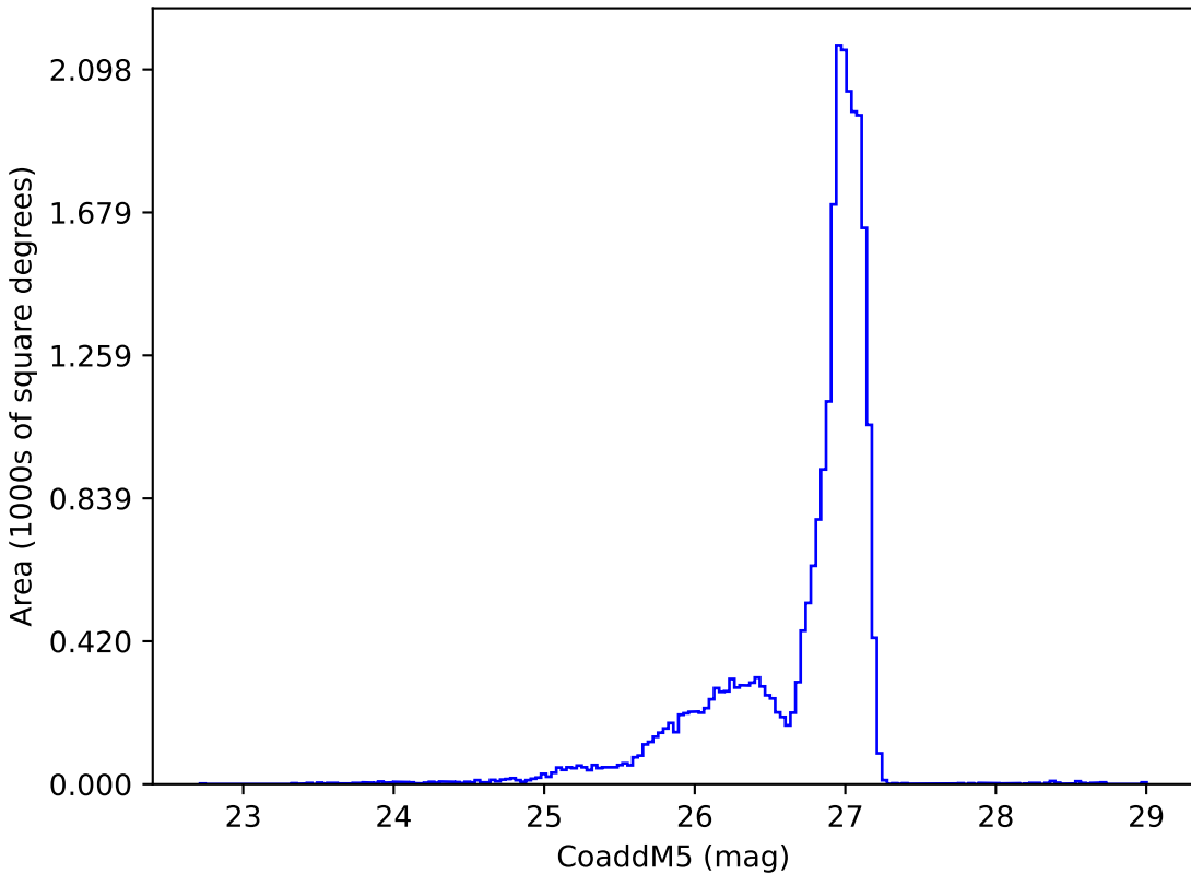
ddf_acor_sf15_lsf20_lsr10_v3.4_10yrs r: CoaddM5
