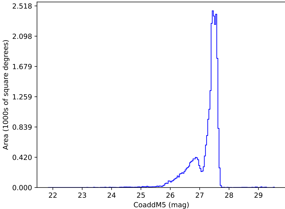
ddf_acor_sf15_lsf20_lsr10_v3.4_10yrs : CoaddM5
